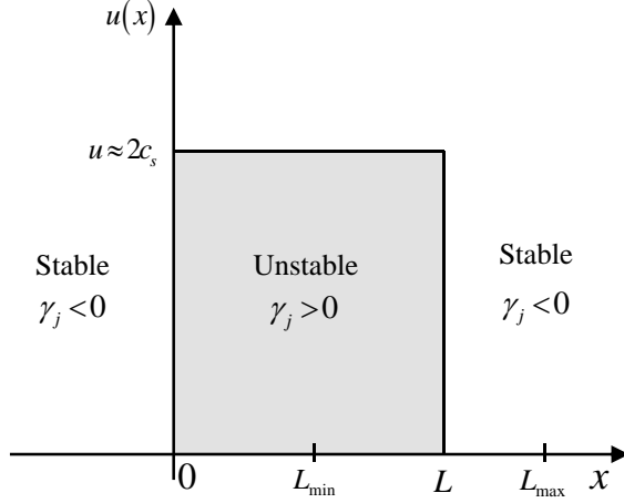
FIG. 2: (Color online) Schematic drawing of the example problem. A finite ion flow of u \sim 2c_s is imposed over a finite region L of the otherwise stable plasma.
