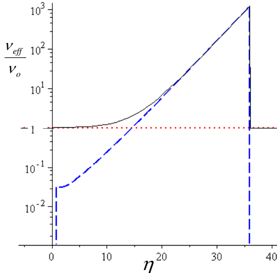
FIG. 4: (Color online) The effective collision frequency, \nu_{eff} , normalized to the reference collision frequency, \nu_o , for Coulomb collisions, i.e., the Lenard-Balescu collision operator (red, dotted line), due to wave particle interactions (blue, dashed line) and the total (black, solid line). Here the ion flow, u \approx 2c_s , is present for 0 < \eta < 35 and is zero otherwise and we have assumed \ln \Lambda = 10 .
