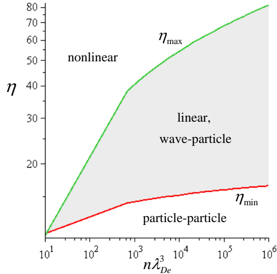
FIG. 3: (Color online) Plot of the maximum dimensionless distance \eta_{max} such that the linear analysis is valid ( \eta < \eta_{max} ) and the minimum dimensionless distance \eta_{min} such that wave-particle interactions dominate the conventional particle-particle scattering. For \eta > \eta_{max} , nonlinear effects may be significant.
